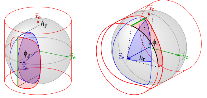
Figure 4: Illustration of our parallel (left) and radial (right) maps. Given a canonical sample (\varepsilon_1, \varepsilon_2) \in [0, 1]^2 , we first find the azimuth angle \phi_p , respectively \phi_r , that cuts a region on the cylindrical ellipse with area \varepsilon_1 \Omega_D (in red, determined by the green line segment). A sample point on the cylinder is then obtained by linearly interpolating the green segment endpoints using \varepsilon_2 . For the parallel map, the endpoint cylindrical coordinates are (\phi_p, -h_p) and (\phi_p, h_p) , with \phi_p \in [-\beta, \beta] . For the radial map, these coordinates are (\phi_r, h_r) and (\phi_r, 1) , with \phi_r \in [0, 2\pi] (we use \phi_r \in [0, \pi/2] in each quadrant).
